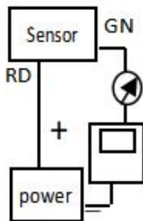
Current output, 2-wire
