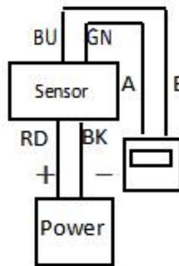
RS485 output
